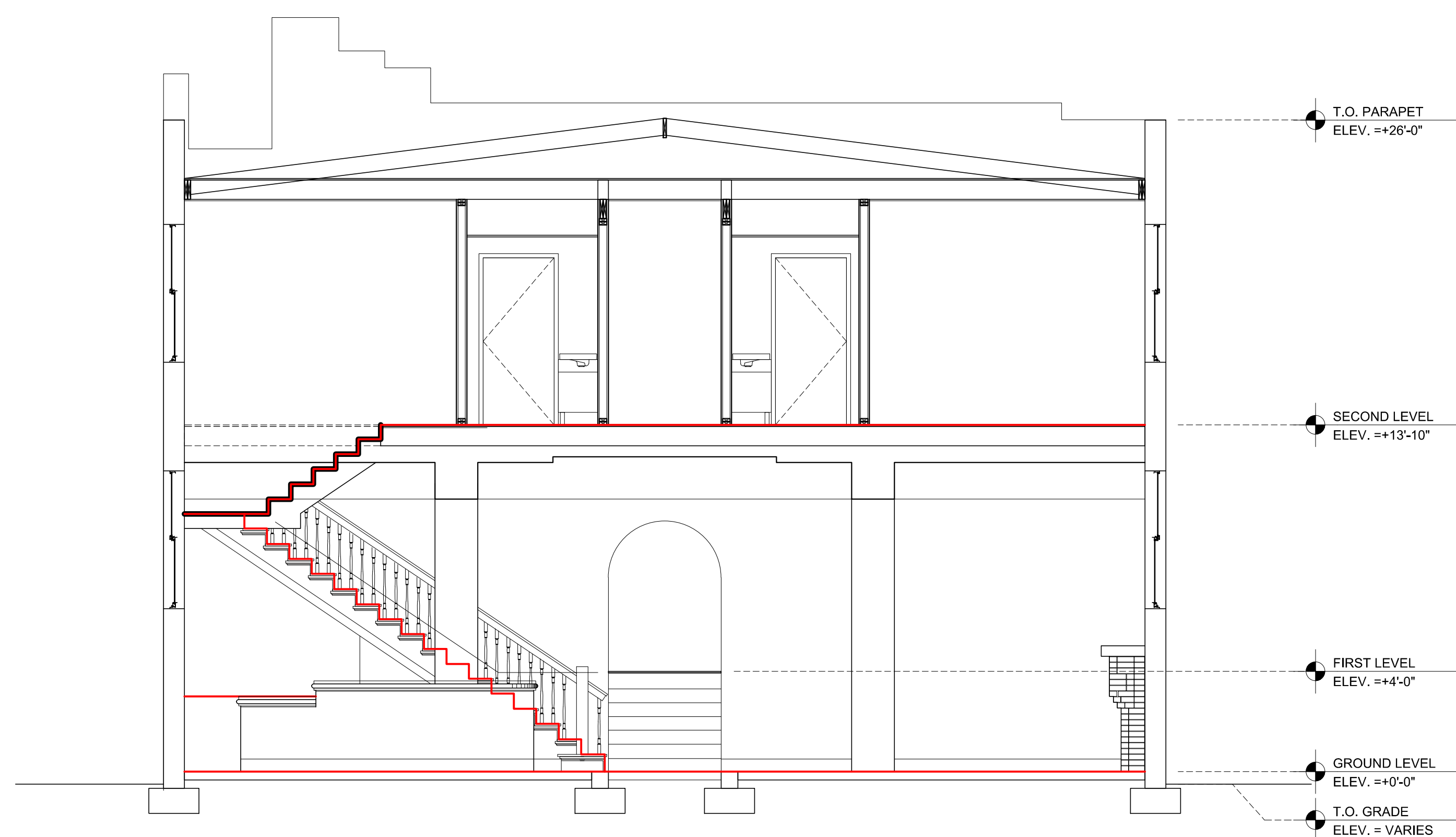
04 PROPOSED SECTION 1/8"=1'-0"
