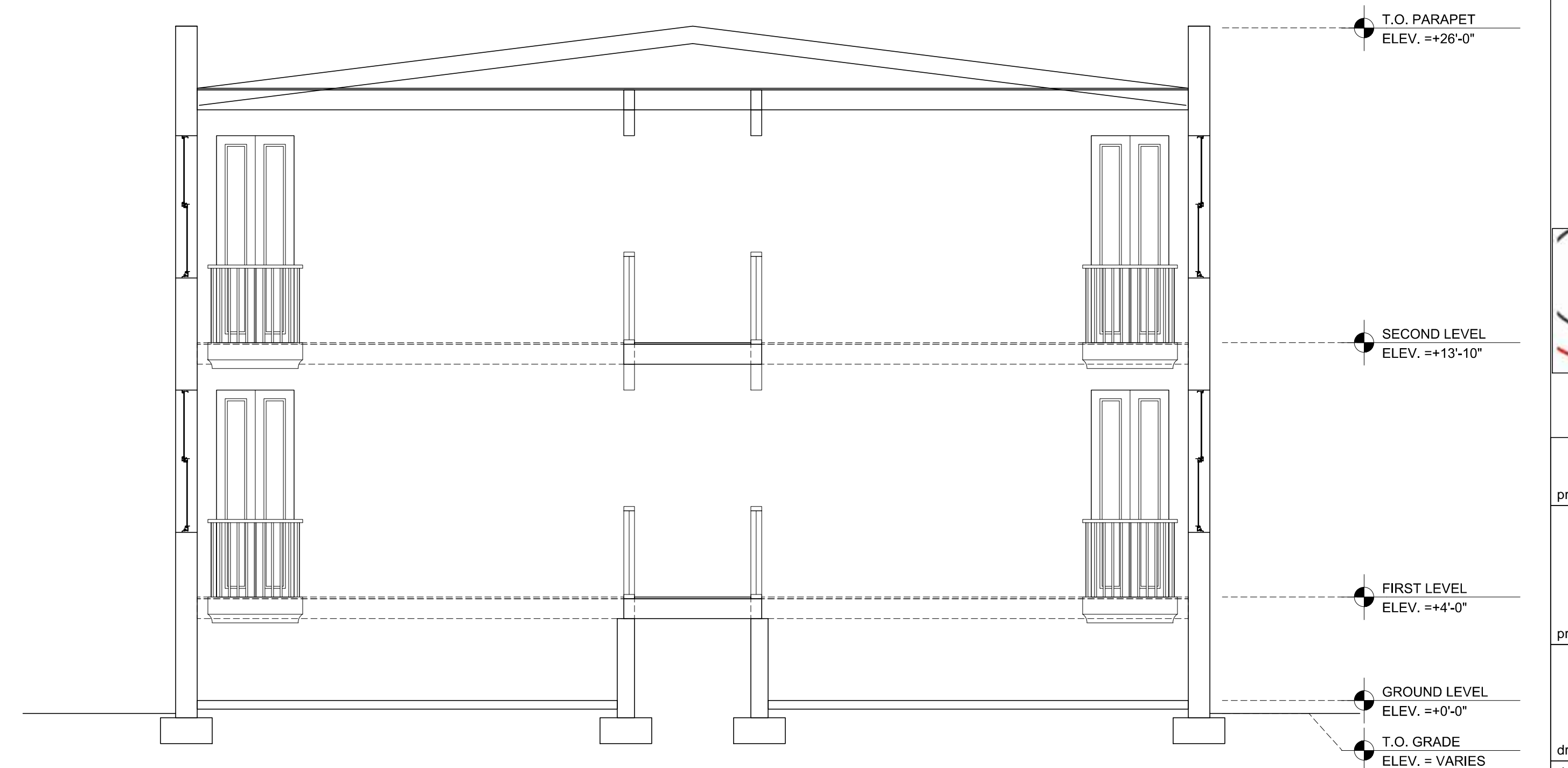
03 PROPOSED SECTION 1/8"=1'-0"
