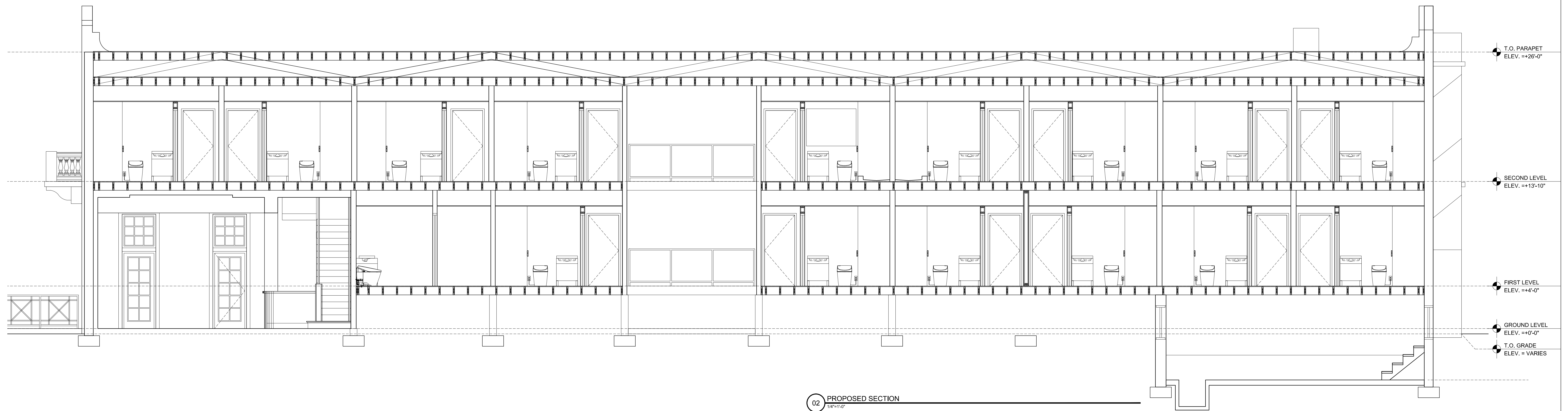
01 PROPOSED SECTION 1/8"=1'-0"
